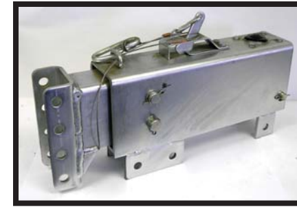
Surge Brake
